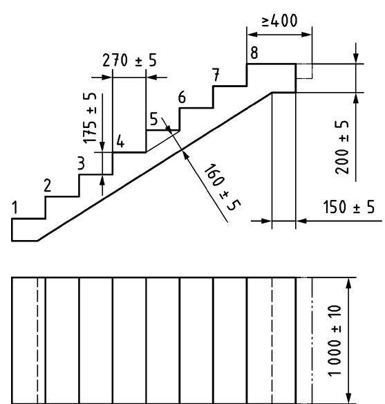
Figure 5 — Dimensions of a reference flight (standard configuration)
