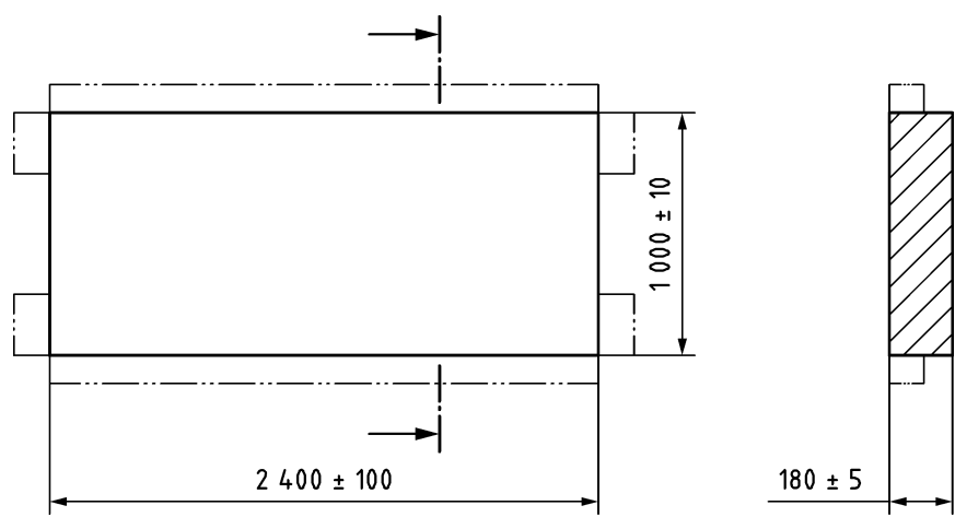
Figure 4 — Dimensions of a reference landing (standard configuration)
